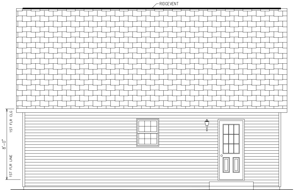
REAR ELEVATION
